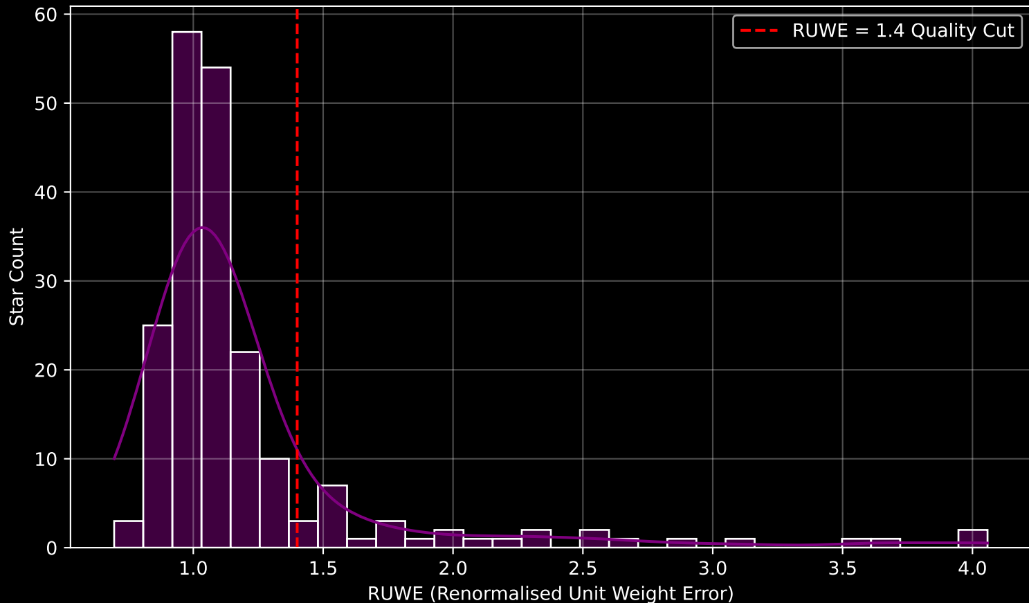
GAPOGEE DR17 Field [046-58-O] RUWE Distribution (n= 202)
