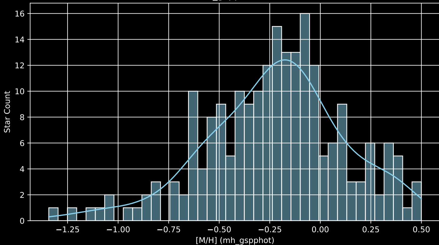
APOGEE DR17 Field: [046-58-O [M/H] (mh_gspphot) (n= 213)
