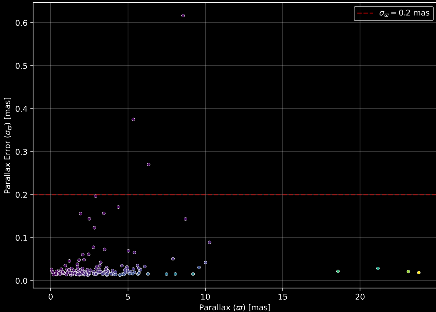
APOGEE DR17 Field: [046-58-O] Parallax Quality (n= 215)
